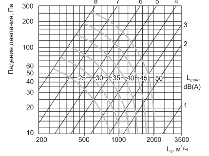
IRIS (SS316)-500
