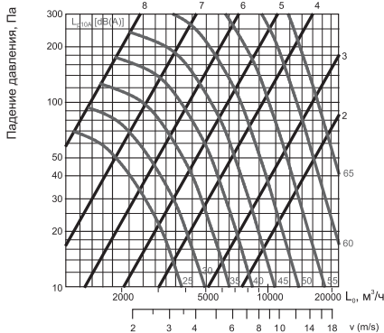
IRIS (SS316)-630
